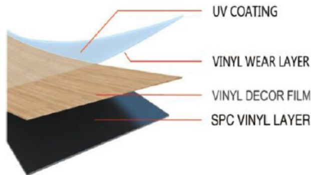
Figure 1. Construction of SPC flooring
