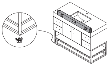
2. Adjusting cabinet foot
