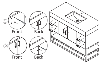
3. Install the handle
